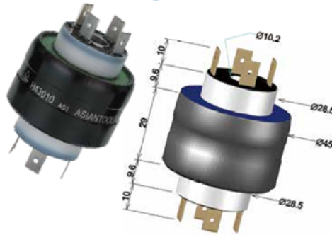
H43010 4poles/30A/AC250V Through-bore:10.2mm
